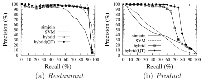
Figure 12: Comparing hybrid human-machine workflow with existing machine-based techniques.
